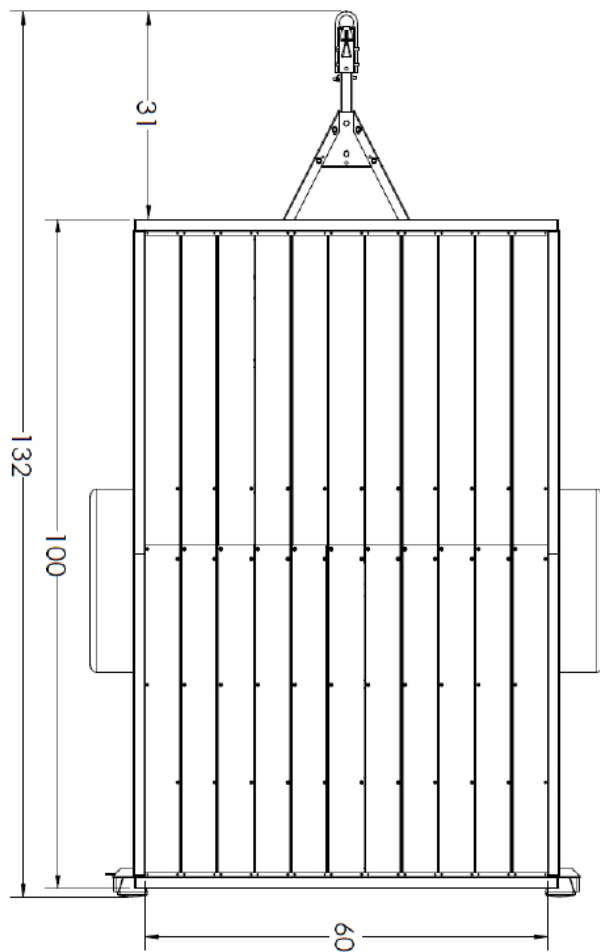
Top View
