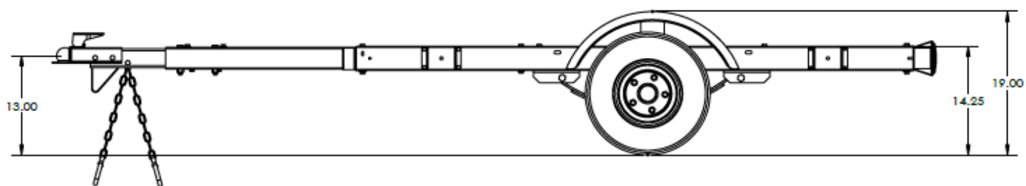
Side View
