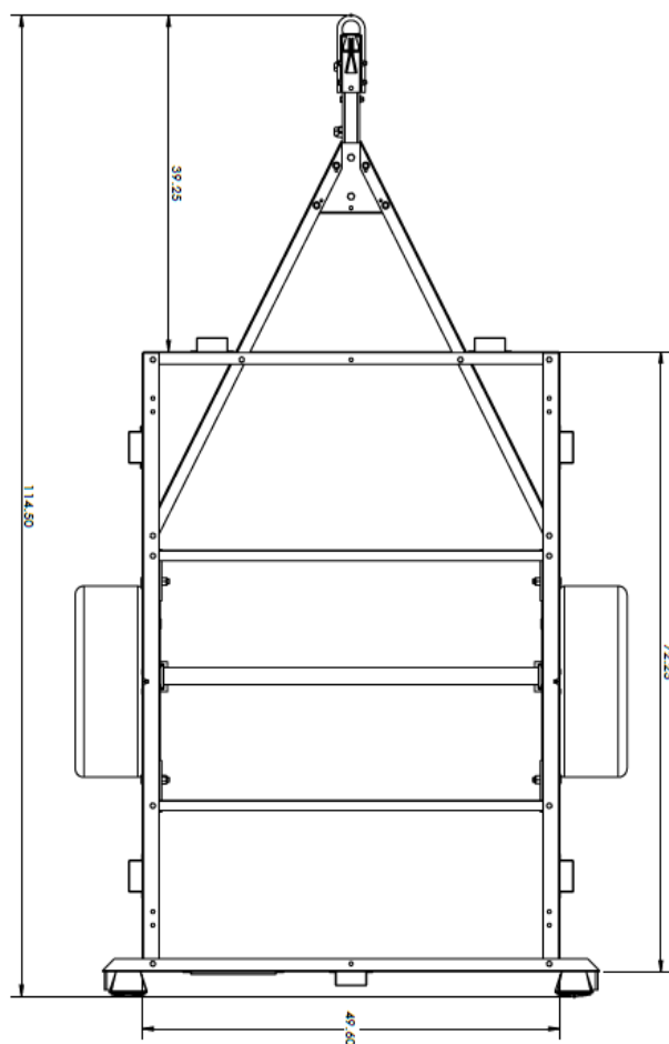
Top View
